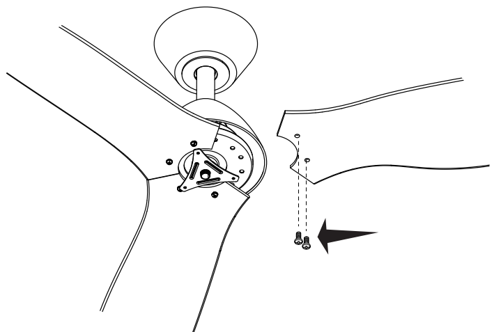
FAN + LED LIGHT MODEL (screw from bottom side)
