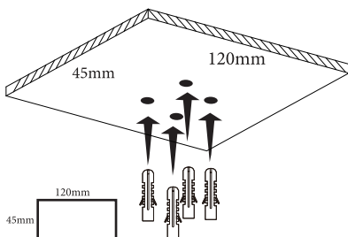
The minimum board size for installing
